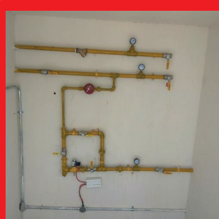
WIRING & EXTENDING COOKING GAS PIPES IN RESIDENTIAL FACILITY & VILLAS
